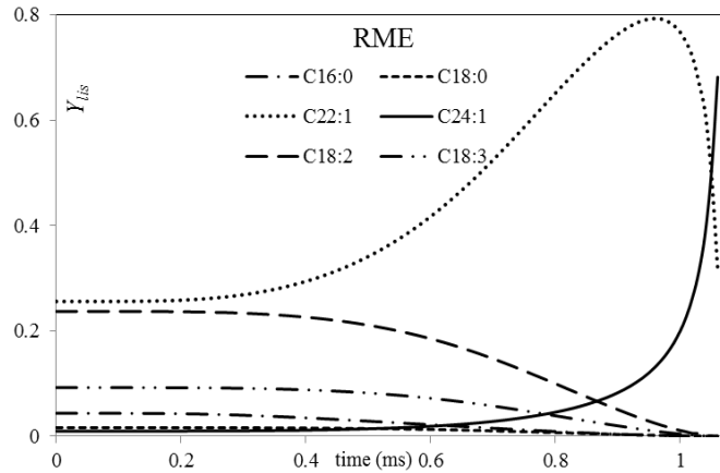
Fig. 3 The plots of time evolution of surface mass fractions of C16:0M, C18:0M, C22:1M, C24:1M, C18:2M and C18:3M for a RME droplet under the same conditions as in Figs. 1 and 2.
