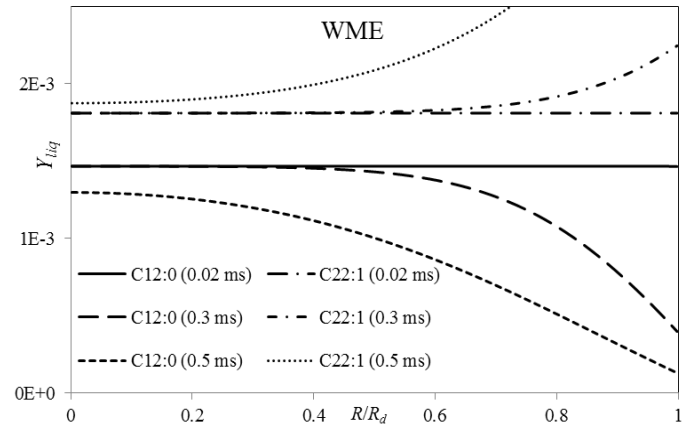
Fig. 6 The plots of mass fractions of C12:0M and C22:1M versus normalised distance from the centre of the droplet at three time instants 0.02 ms, 0.3 ms and 0.5 ms for a WME droplet under the same conditions as in Figs. 1-5.
